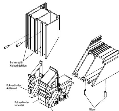
Eckverbinder Set Tür (p/n)
