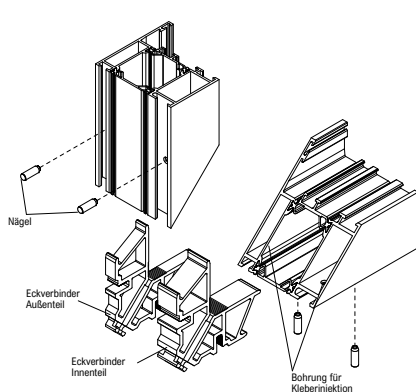
Eckverbinder Set Fenster (p/n)
